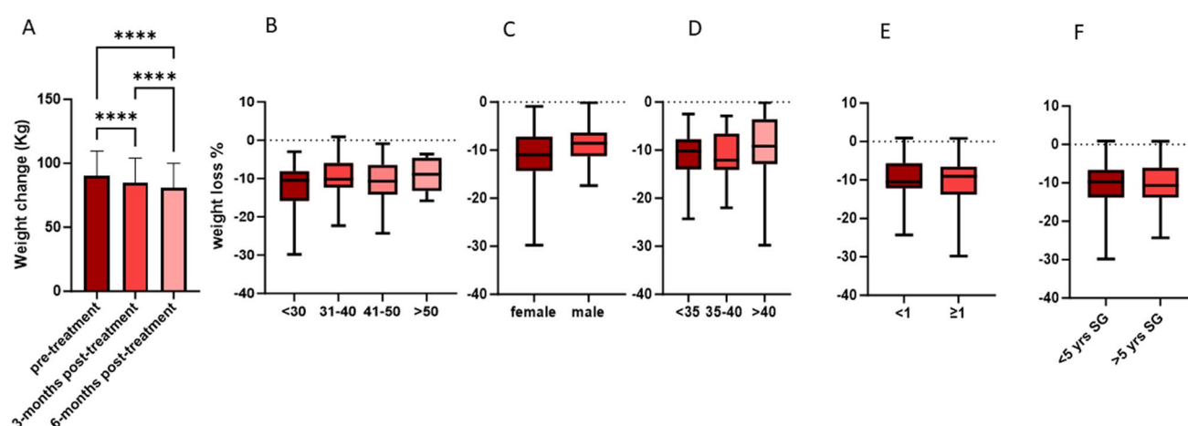
Fig. 2 Post-treatment weight change at 6 months of semaglutide patients. A For all patients, B by age groups, C by gender the duration of treatment, D by BMI, E by maximum-tolerated dose, and F by SG duration
